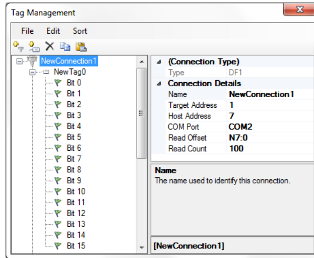
Figure 11 - Tag Management window
