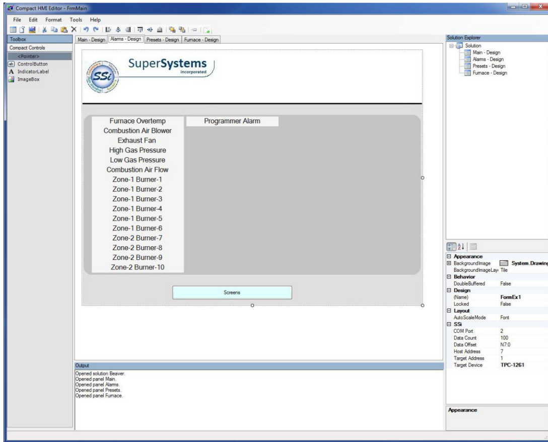
Figure 50 - Alarms Panel (Compact HMI Editor)
