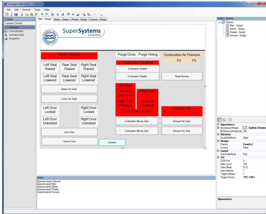
Figure 47 - Main Panel (Compact HMI Editor)
