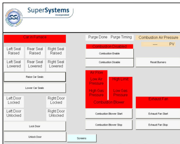
Figure 48 - Main Panel (Compact HMI - Touch Screen)
