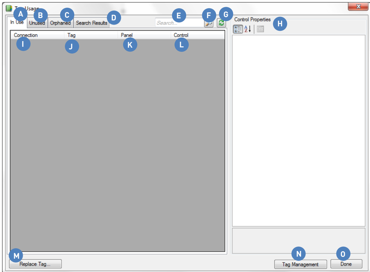
Figure 23 - Tag Usage window
